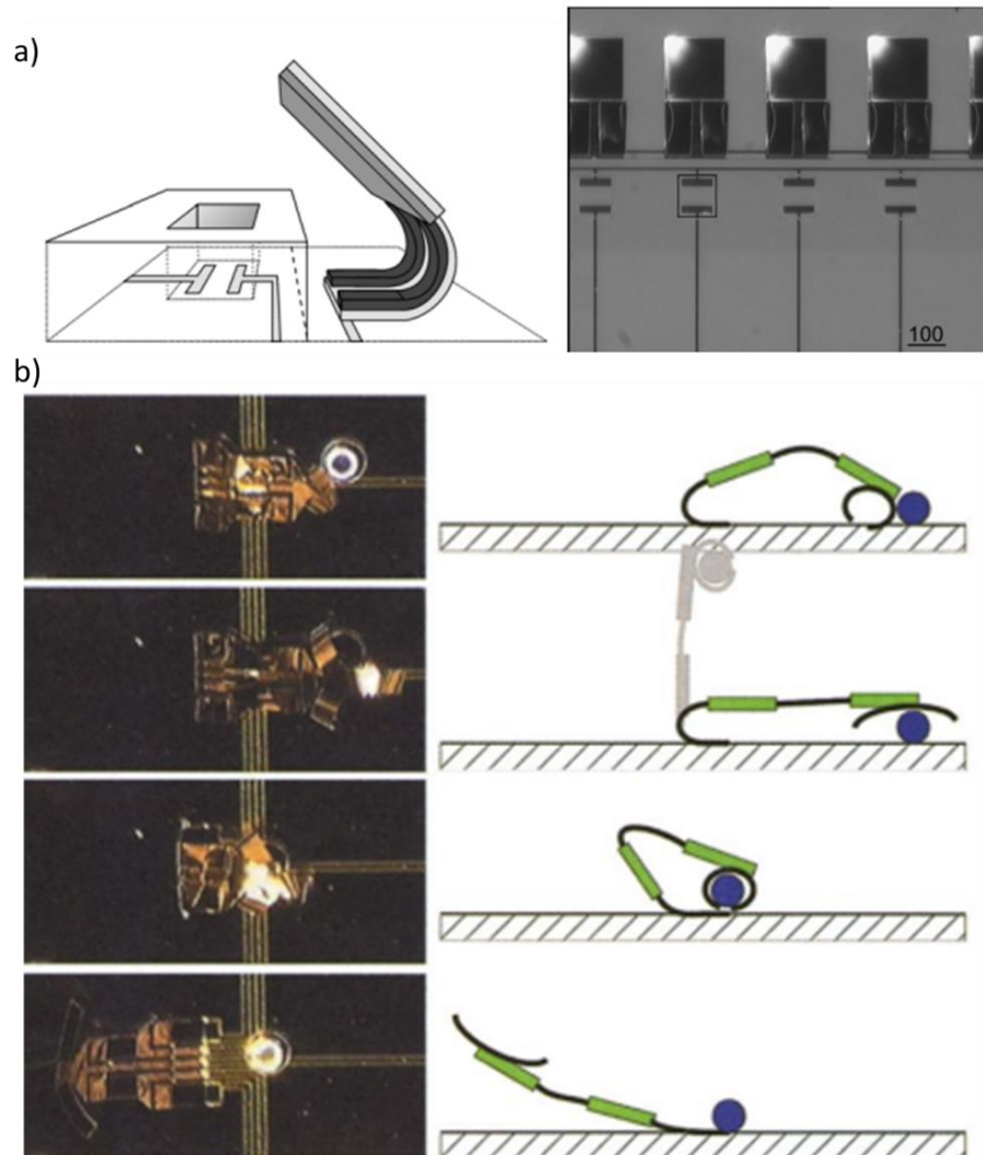
Fig. 6. a) A schematic drawing of a closable microvalves [16] (Reprinted with permission from Springer Nature), b) A sequence of pictures (left) showing the grabbing and lifting of a 100 μm glass bead and schematic drawings of the motion (right) [17] (Reprinted with permission from The American Association for the Advancement of Science)
