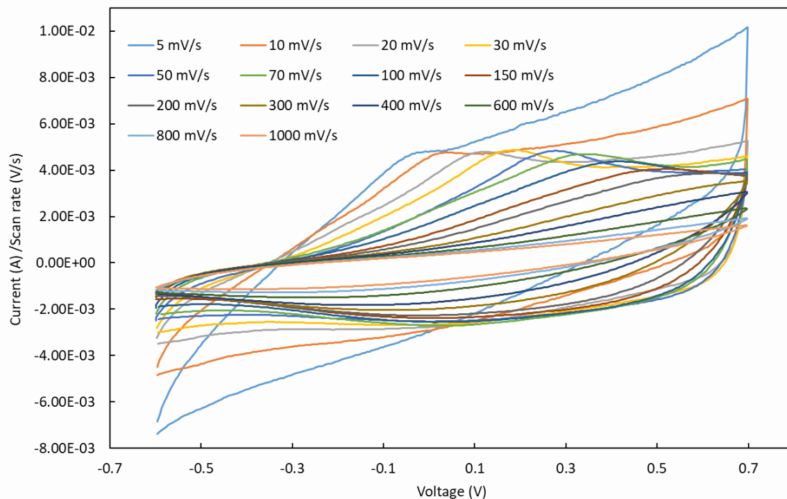
Fig. 6 Cyclic voltammograms of PEDOT electrodes obtained in neat EMImTFSI within a potential window of -0.6 V to +0.7 V with different scanning rates. The vertical axis indicates the current (A) scaled by the scanning rate (V/s).
