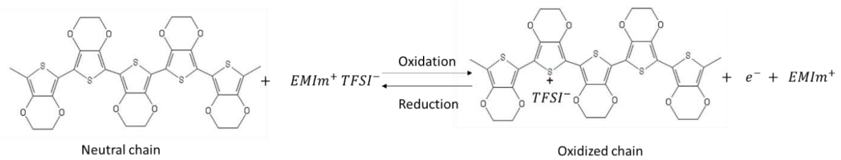
Fig. 2. Cation driven actuation in a PEDOT-based actuator.
