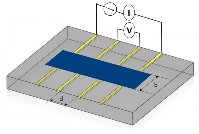
Fig. 5. A built in-house four-line probe to measure the electronic conductivity of the PEDOT electrodes, where the distance between two copper lines is d = 2 mm.
