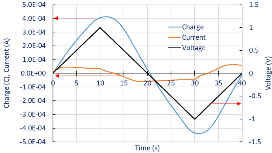
Figure 16. Current and charge response to a triangular input voltage.
